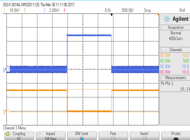
ON/OFF 起机波形 (负逻辑) CH1:输出电压 CH2:ON/OFF 引脚电压
