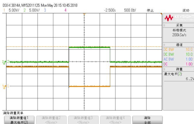
ON/OFF 起机波形 (负逻辑) CH1:输出电压 CH2:ON/OFF 引脚电压
