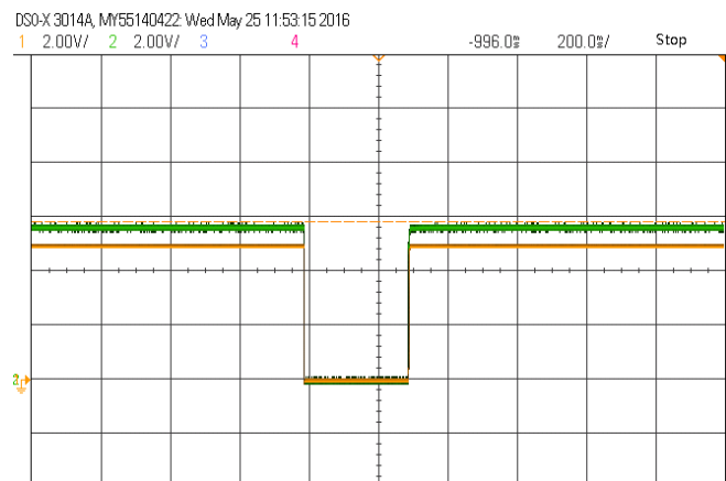
ON/OFF 起机波形 (正逻辑) CH1:输出电压 CH2:ON/OFF 引脚电压
