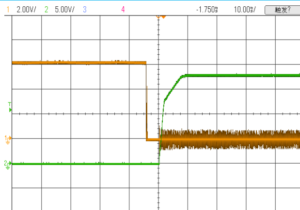
ON/OFF 起机波形 (负逻辑) CH1: ON/OFF 引脚电压 CH2: 输出电压
