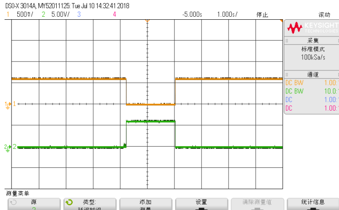
ON/OFF 起机波形 (正逻辑) CH1:输出电压 CH2:ON/OFF 引脚电压
