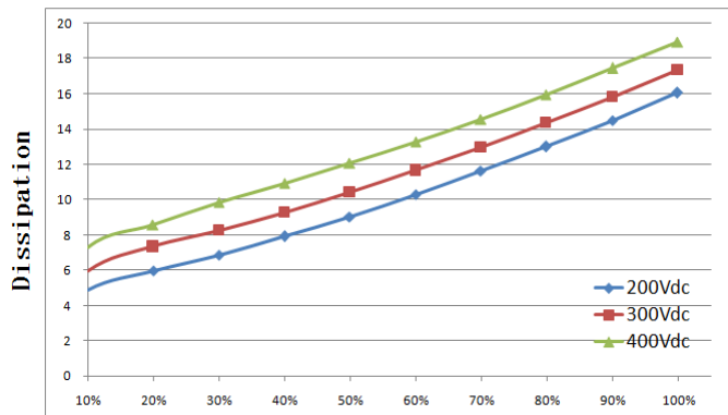
Dissipation VS Load
