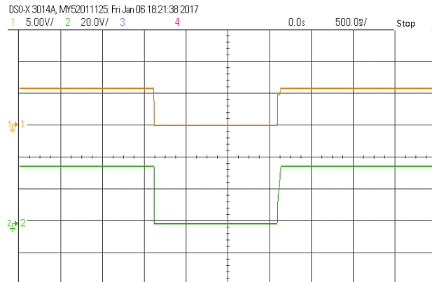
ON/OFF 起机波形 (正逻辑) CH1:输出电压 CH2:ON/OFF 引脚电压
