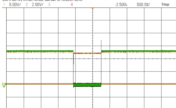
ON/OFF 起机波形 (负逻辑) CH1:输出电压 CH2:ON/OFF 引脚电压
