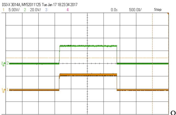
N/OFF 起机波形 (正逻辑) CH1: ON/OFF 引脚电压 CH2: 输出电压
