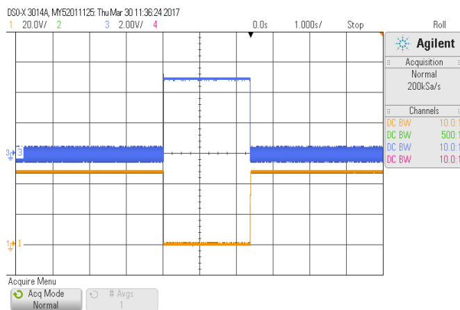
ON/OFF 起机波形 (负逻辑) CH1:输出电压 CH2:ON/OFF 引脚电压
