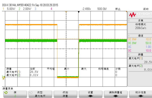
ON/OFF 起机波形 (正逻辑)
