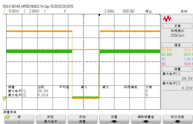
ON/OFF 起机波形 (负逻辑)
