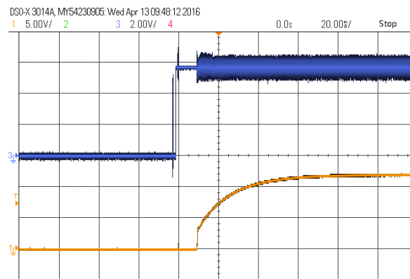
ON/OFF 起机波形 (负逻辑) CH3:ON/OFF 引脚电压 CH1:输出电压
