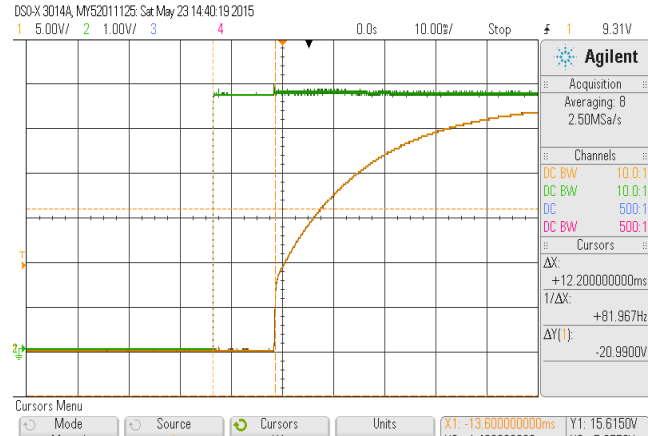
ON/OFF 起机波形 (正逻辑) CH2:ON/OFF 引脚电压 CH1: 输出电压
