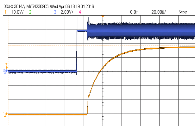
ON/OFF 起机波形 (正逻辑) CH3:ON/OFF 引脚电压 CH1:输出电压
