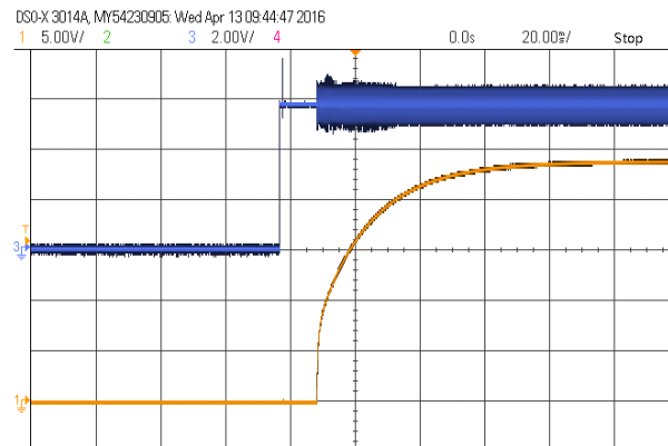
ON/OFF 起机波形 (正逻辑) CH3: ON/OFF 引脚电压 CH1: 输出电压
